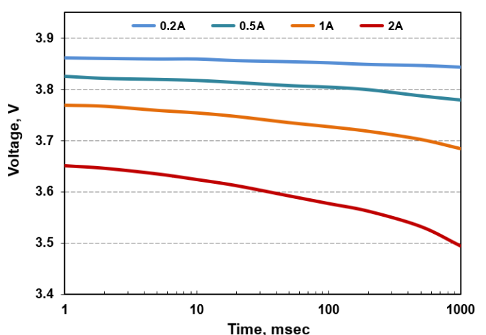
Voltage curves at RT for HLC-1020P6 at Li/SO 2 Cl 2 potential (3.90V)
