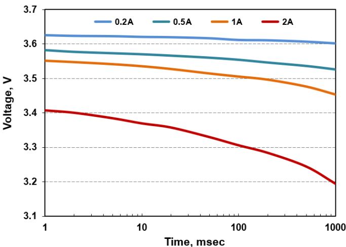
Voltage curves at RT for HLC-1020P6 at Li/SOCl 2 potential (3.67V)
