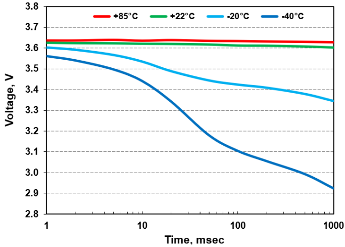
Voltage curves for HLC-1020P6 at Li/SOCl 2 potential (3.67V), 200 mA
