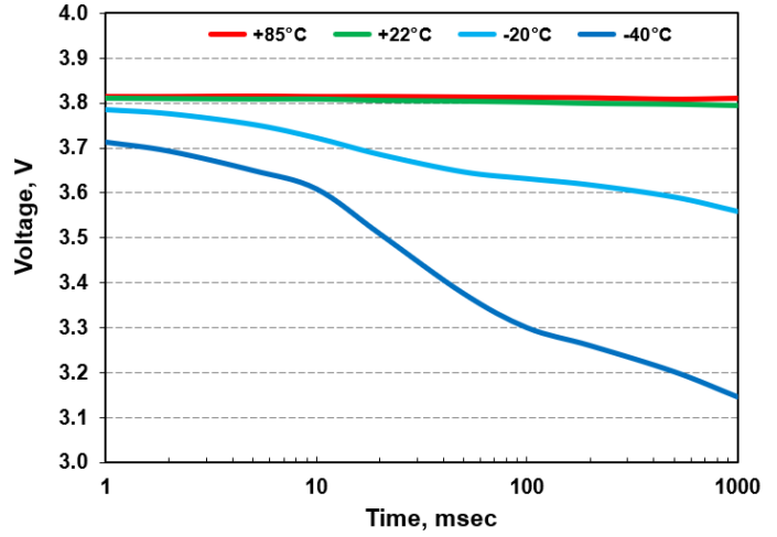
Voltage curves for HLC-1020P6 at Li/SO 2 Cl 2 potential (3.90V), 200 mA
