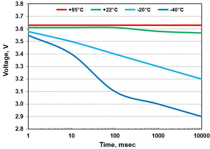
Voltage curves for HLC-1530B at Li/SOCl 2 potential (3.67V), 350 mA
