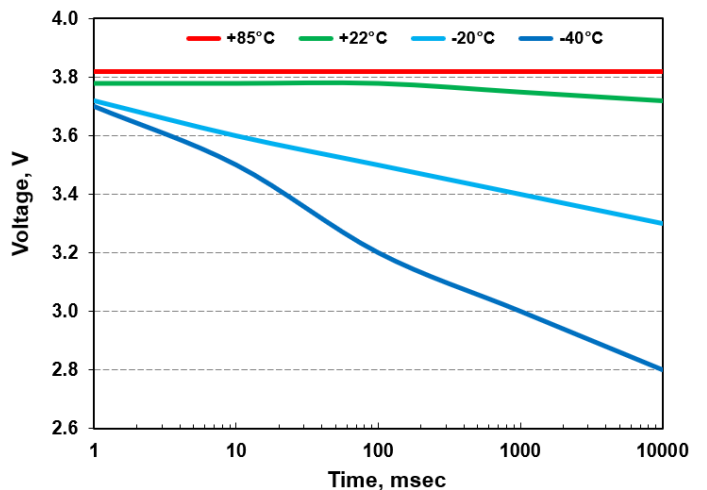
Voltage curves for HLC-1530B at Li/SO 2 Cl 2 potential (3.90V), 600 mA
