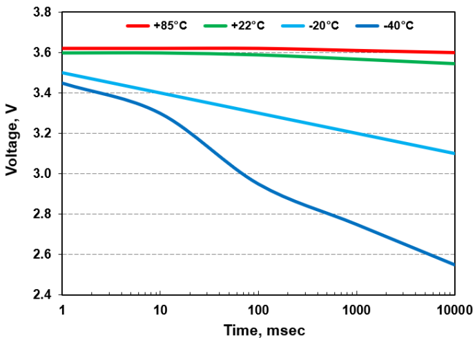
Voltage curves for HLC-1530B at Li/SOCl 2 potential (3.67V), 600 mA
