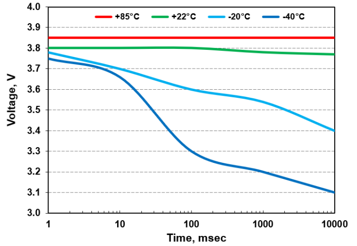
Voltage curves for HLC-1530B at Li/SO 2 Cl 2 potential (3.90V), 350 mA
