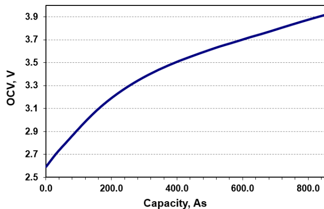
Discharge capacity vs. OCV for HLC-1550A (at RT, 200 mA discharge)
