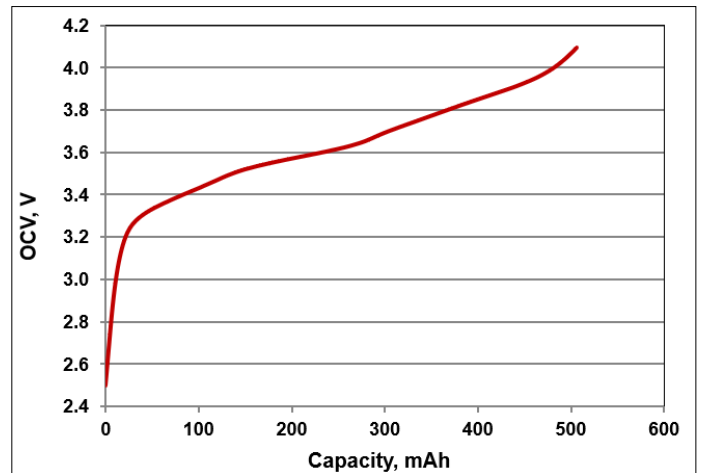
OCV vs Capacity
