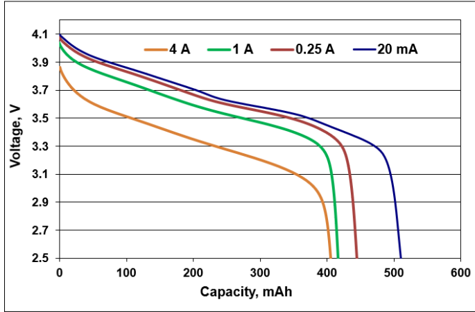
Discharge curves at Room Temperature
