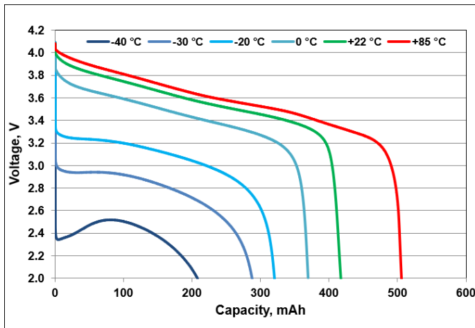
Discharge curves at 1 A
