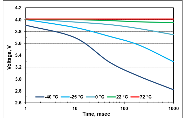
Voltage Curves at 1 A
