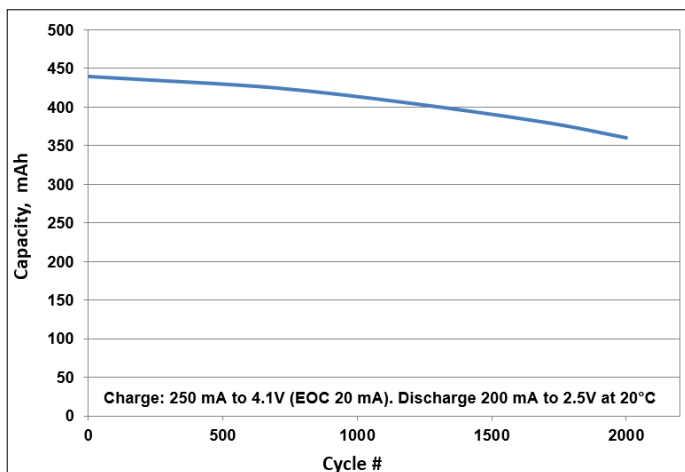
Charge / Discharge Cycling Performance
