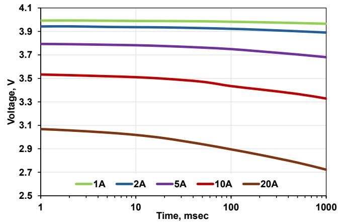
Pulse capability at room temperature, 4.05 V potential
