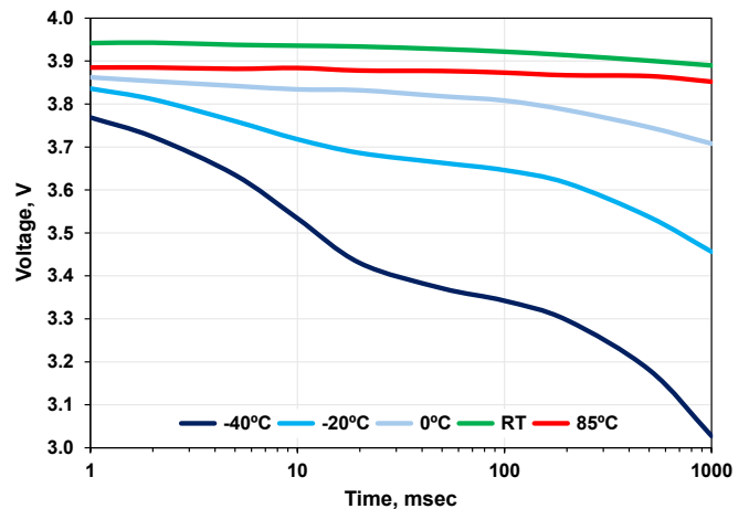
Pulse capability at 2 A, 4.05 V potential
